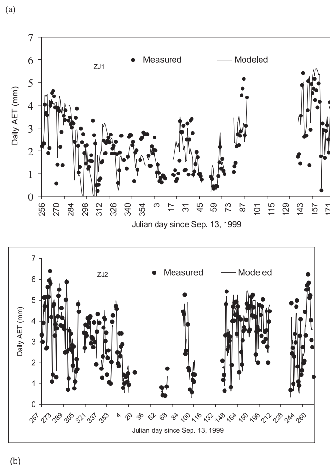
FIGURE 2. Modeled and Measured Daily Actual Evapotranspiration, E , in Zhanjiang 1 (ZJ1) and Zhanjiang 2 (ZJ2) Sites During 13-Sept-1999 to 23-Sept-2000. Some data were missing as a result of lighting-induced equipment failures.
