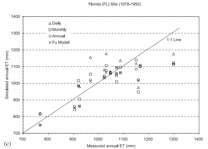
FIGURE 6. A Comparison of Measured Annual ET and Simulated Total Annual ET by Three Methods at (a) Coweeta (CW), (b) Carteret (CT), and (c) Florida (FL) Sites in the Southern U.S.
