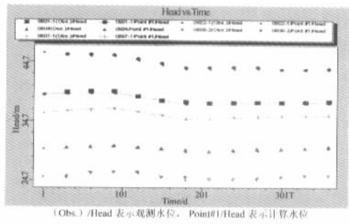
图 5 栾城县地下水位计算值与观测值的拟合情况 Fig. 5 Fitting curve of the calculating data and observation data in Luancheng county
